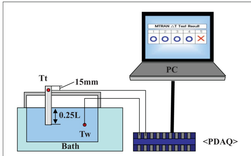
Fig. 7 Thermal Response Test Apparatus
