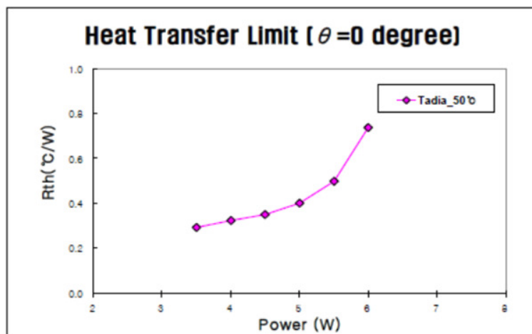
Fig. 3 Maximum Heat Transfer Rate at \theta=0^\circ , Tadia=50°C ( L_e=28\text{mm} , L_a=30\text{mm} , L_c=67\text{mm} )
