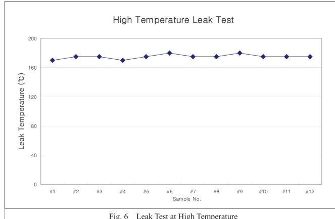
Fig. 6 Leak Test at High Temperature
